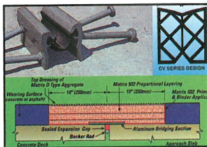
Expansion Joints
